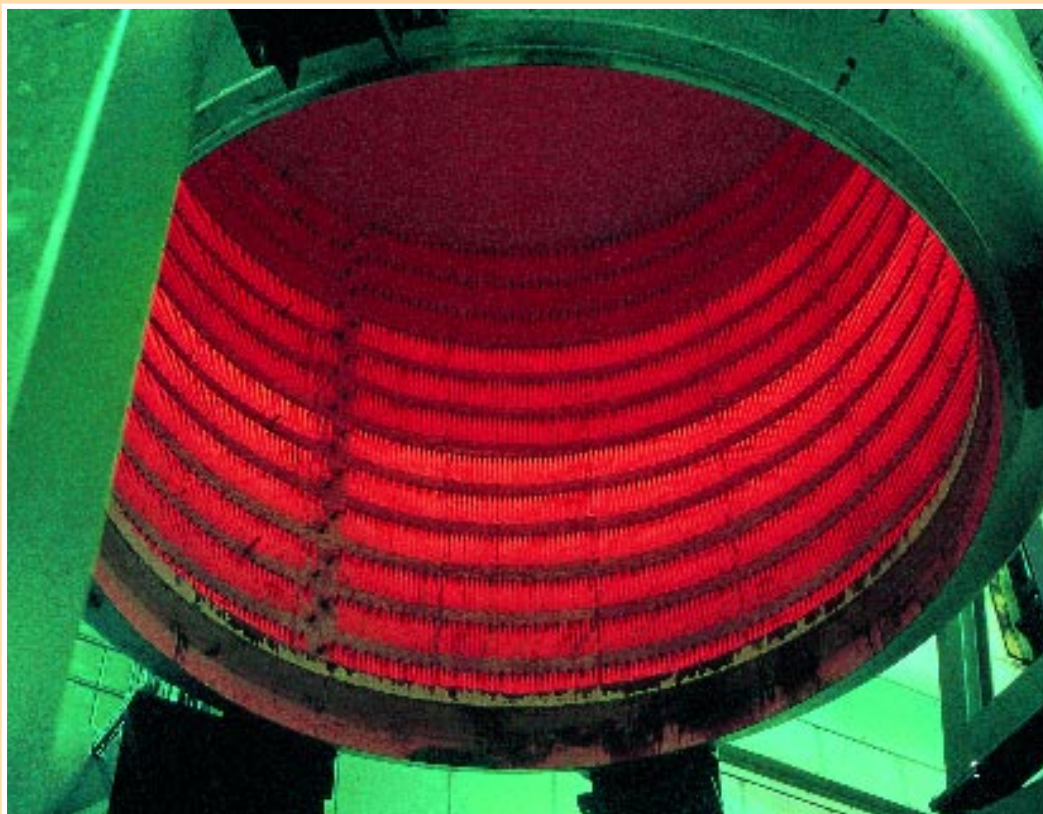
Fig. 31. ROB-Modules in a Bell furnace
