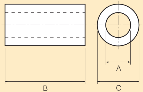
Fig. 10. FIBROTHAL Half-cylinders
