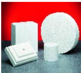
Fig. 7. Insulation parts of vacuum-formed fibre in the most varied shapes for application temperatures up to 1800°C
