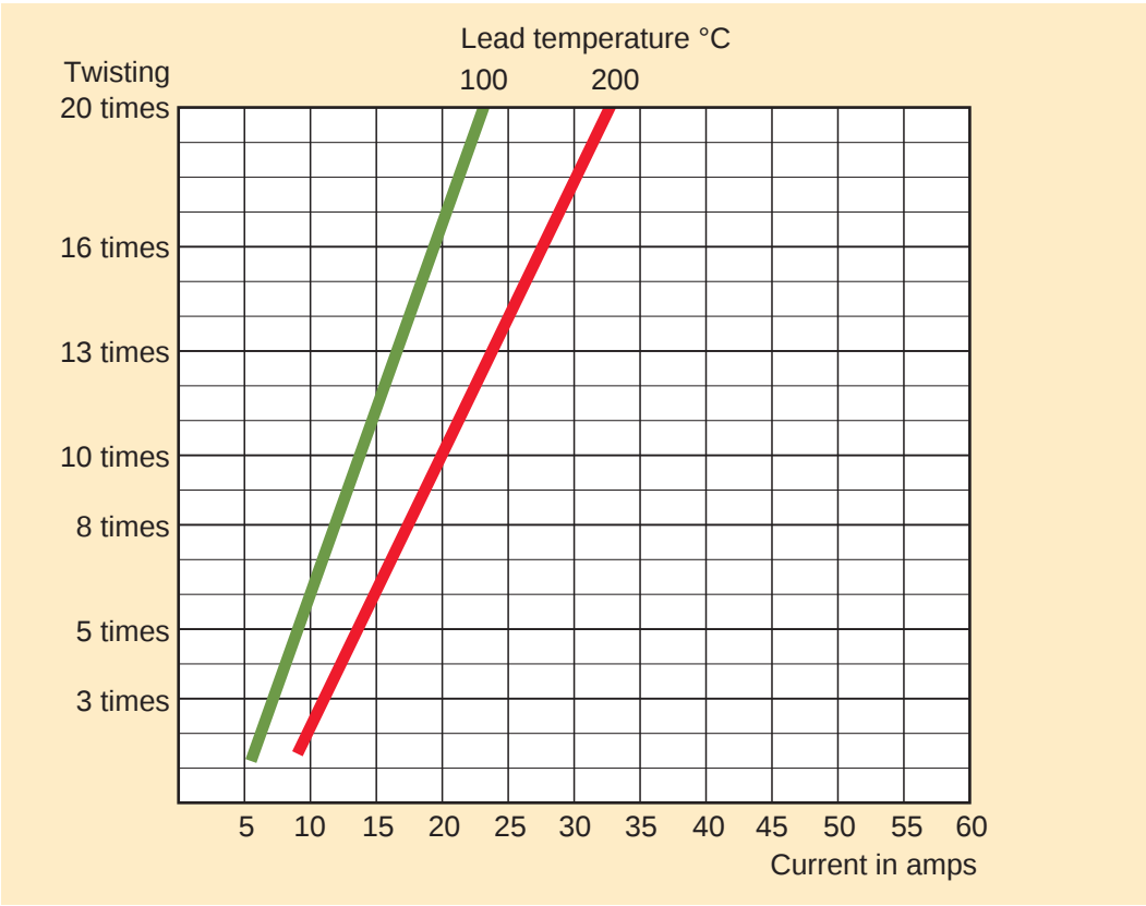
Fig. 29. Leads bead-insulated in Fibrothal
