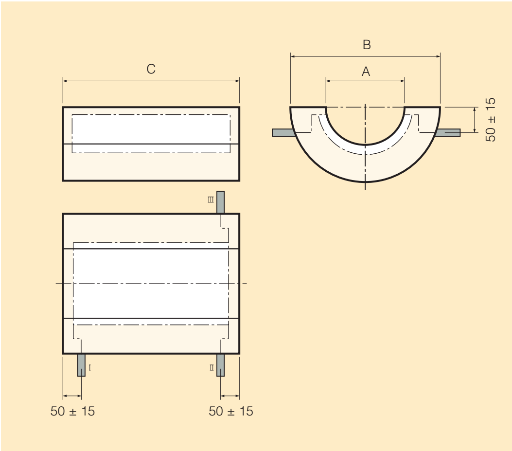
Fig. 18. FIBROTHAL Standard half-cylinders
